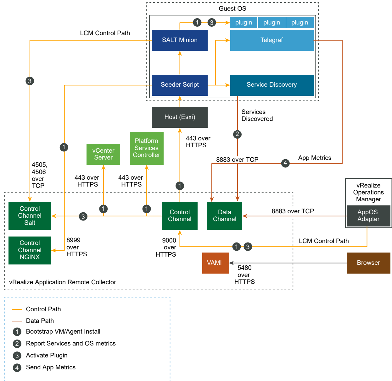
Figure 2-1. Port Information and Communication with vRealize Operations Manager, vCenter Server, and the End Points
