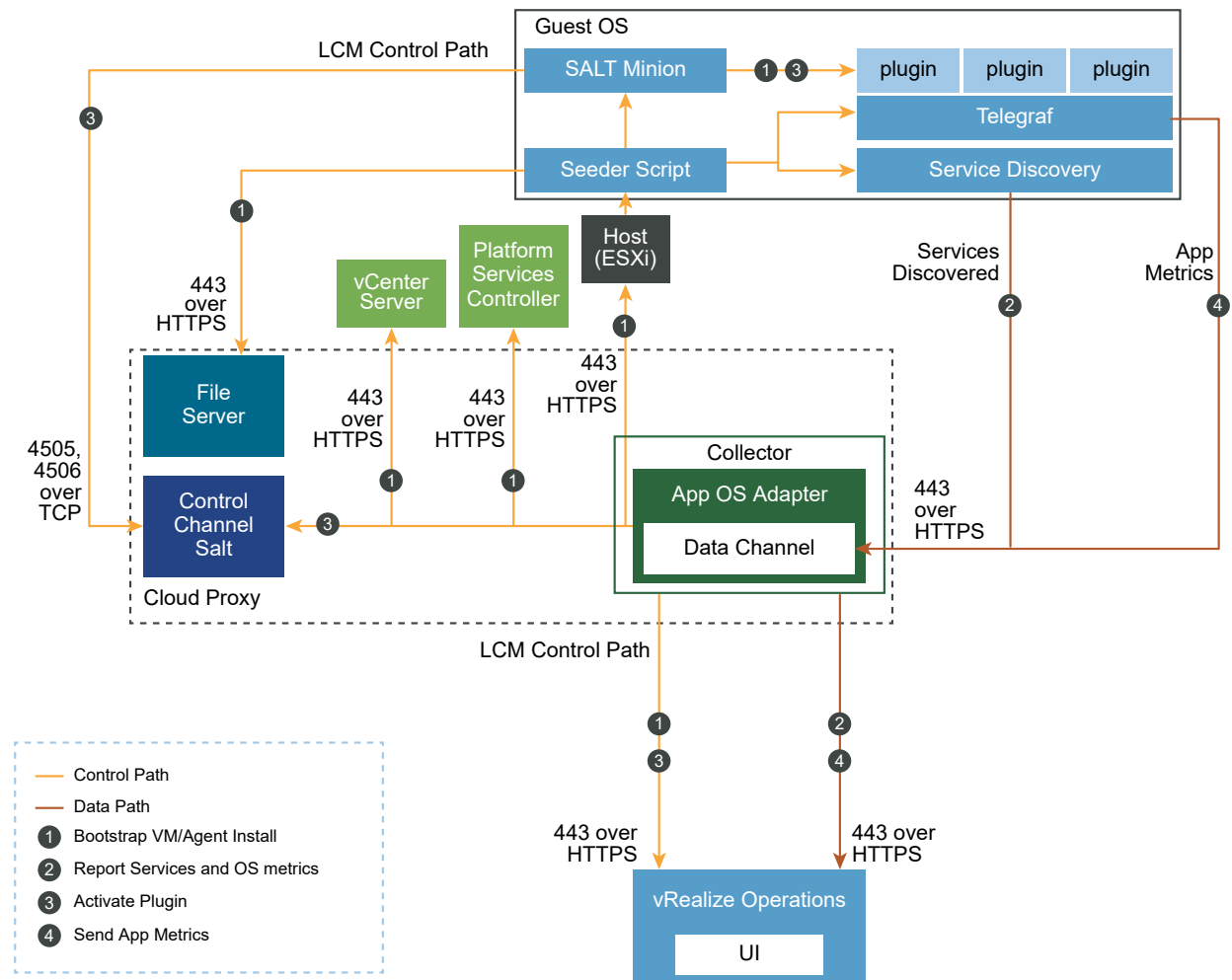
Figure 2-2. Port Information and Communication with vCenter Server and the End Points (Agent Install from the UI)
