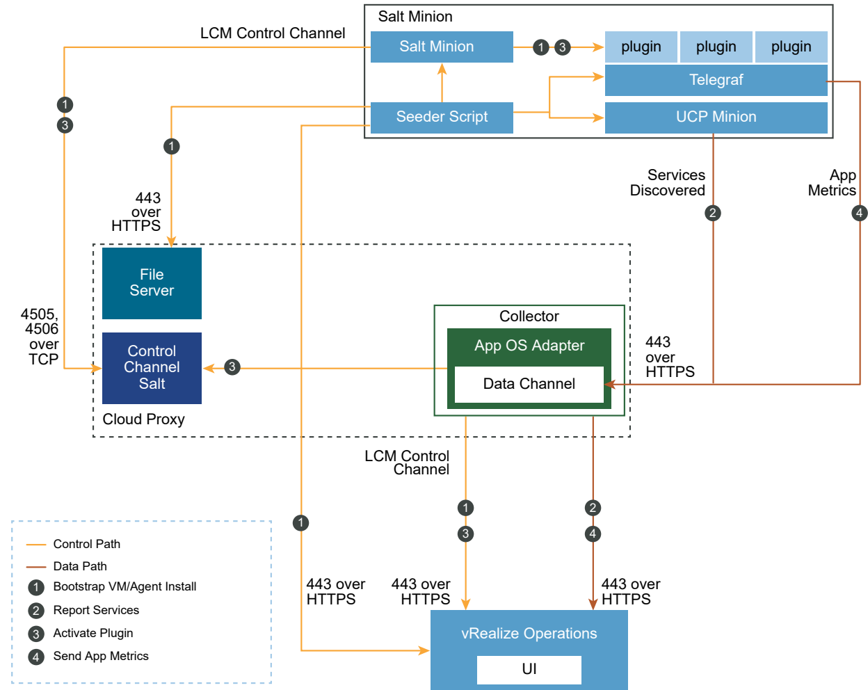
Figure 2-3. Port Information and Communication with the End Points for Script-Based Agent Install
