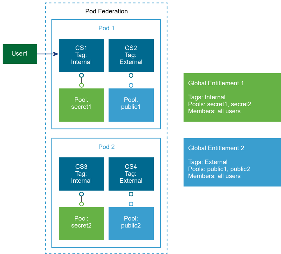
Figure 2-2. Connection Server Restrictions Example
